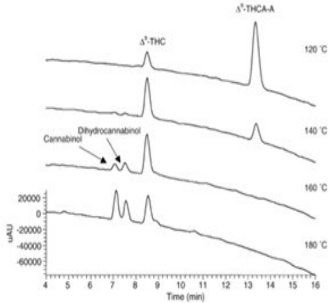
Fig. 8. Conversion of \Delta^9 -THCA-A into \Delta^9 -THC prior to HPLC analysis.
