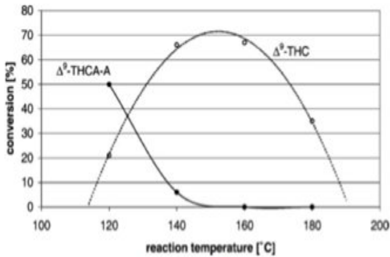
Fig. 8. Conversion of \Delta^9 -THCA-A into \Delta^9 -THC prior to HPLC analysis.
